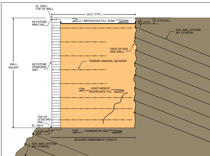
Cross section shows soil nailed bluff below and geogrid soil reinforced Keystone above.
